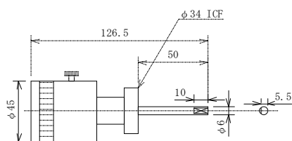
NF-R-34SB
