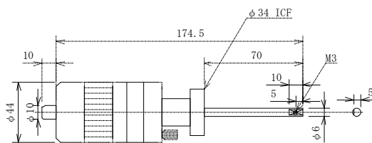
NF-R-34HB
