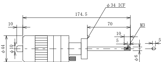
NF-R-34HB
