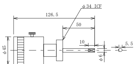
NF-R-34SB
